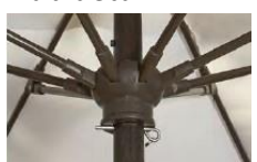
Hub detail
